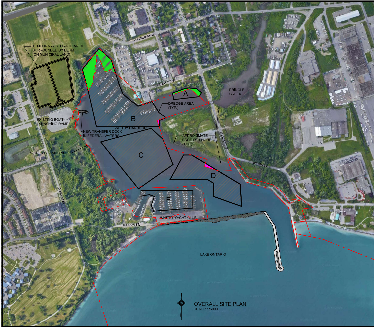
FIGURE 1 OVERALL SITE PLAN
